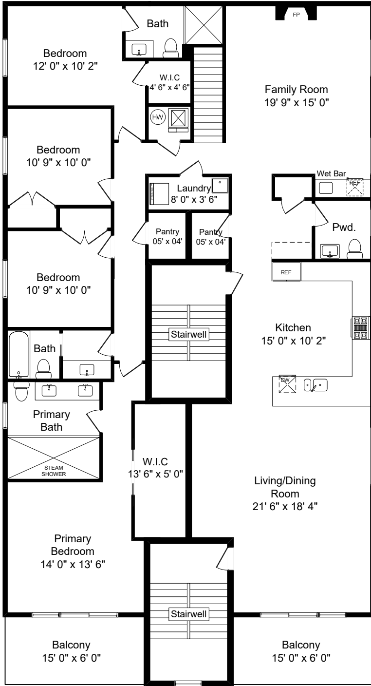
FOURTH FLOOR
