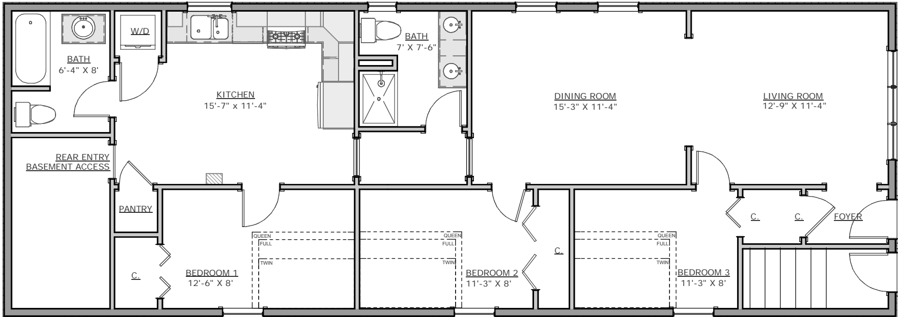
FLOOR PLAN - 1st FLOOR UNIT
